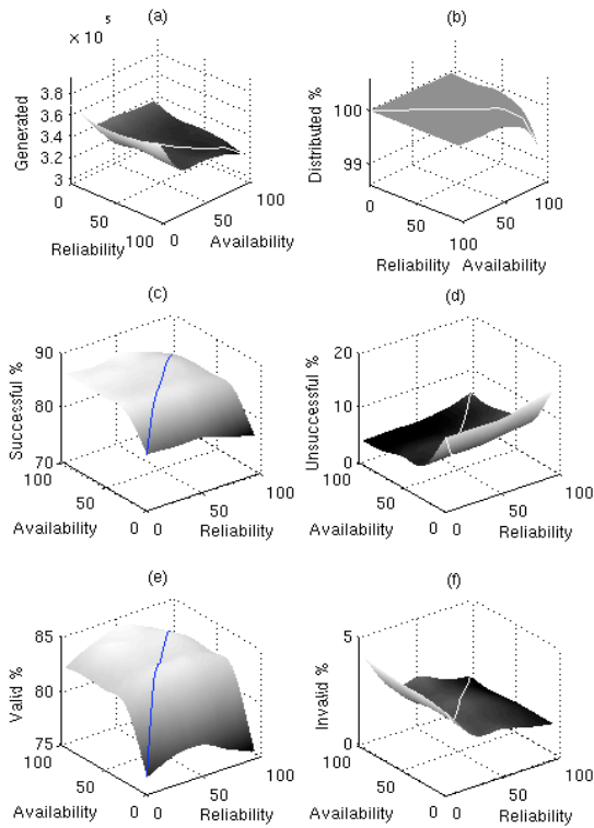
MFold Application
