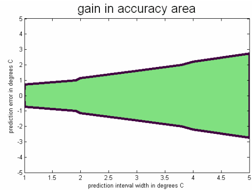
Figure 14. Dependence of the possible gain area with four temperature sensors on the prediction error and the prediction fuzziness (prediction interval width in degree Celcius)
