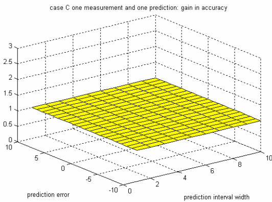
Uniform measurement distribution and approximate prediction
