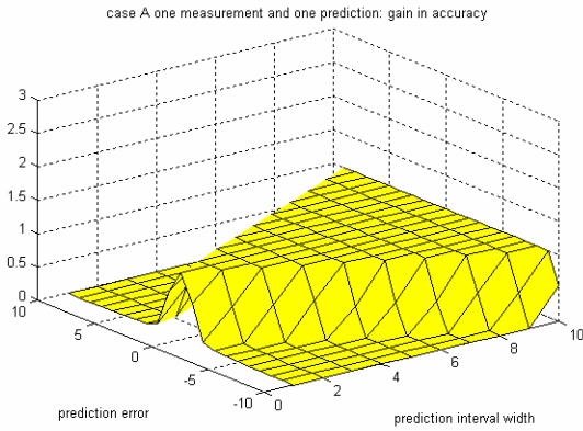
Uniform measurement distribution and interval prediction
