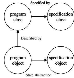
Figure 1: A specification reflection model
