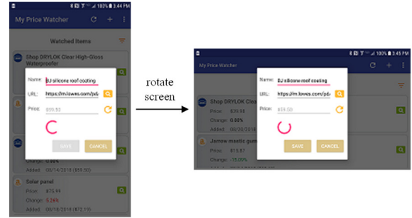
Figure 4. Screen orientation change
