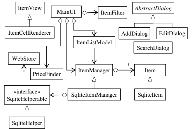
Figure 2. Design of the Java version
