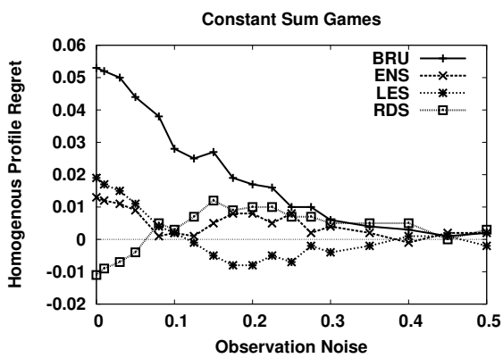
Figure 5: Comparison of four classes of meta-strategies across different noise levels for six combinations of game class and observation model. The stochastic observation model results are on the left, and the incomplete observation model on the right.
