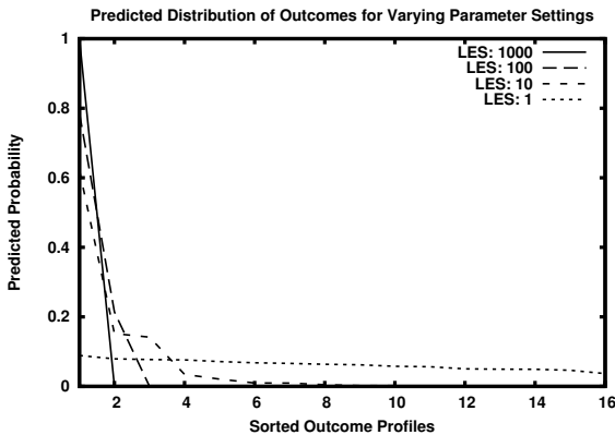
Figure 3: As the LES parameter \lambda is decreased, the predicted outcome distributes weight more evenly across the outcomes. Each line shows a distribution where outcomes are first sorted by probability, so the probability associated with the most likely outcome is on the far left.
