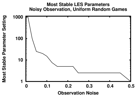
Figure 4: The parameter settings for ENS, RDS, and LES with the most stable homogeneous profiles for different noise levels. Results are shown for both the stochastic and incomplete observation models on random games. For ENS and RDS, higher parameter settings correspond to less specific predictions, while higher settings for LES correspond to more specific predictions.
