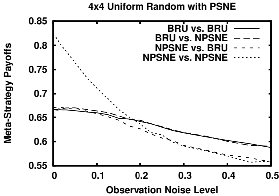
Figure 2: Payoffs to NPSNE and BRU with varying noise levels, for random games and stochastic observations.
