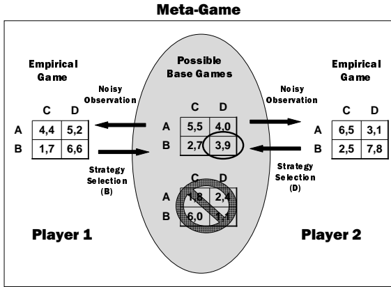
Figure 1: A graphical depiction of a meta-game showing selection of the base game, generation of empirical games, and strategy selections based on the empirical games. Here, player 1 chooses strategy B and receives payoff 3, while player 2 chooses strategy D and receives payoff 9.
