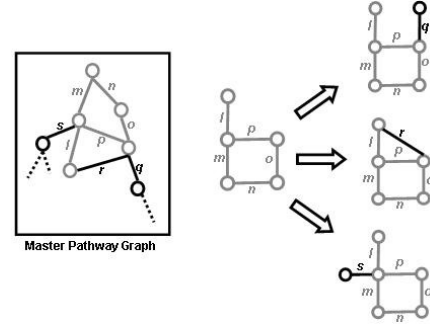
Figure 4. 6-edge Subgraph-Extension Generation for the 5-edge subgraph lmnop .
