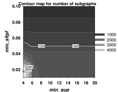
Figure 8. Contour map illustrating number of generated subgraphs.
