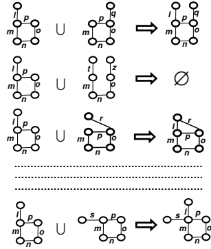
Figure 3. Attempts to combine lmnop with other 5-edge subgraphs of L_5 .
