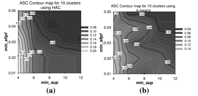
Figure 12. Contour map for ASC at 10 clusters (a) Hierarchical Agglomerative (b) k-means Clustering.
