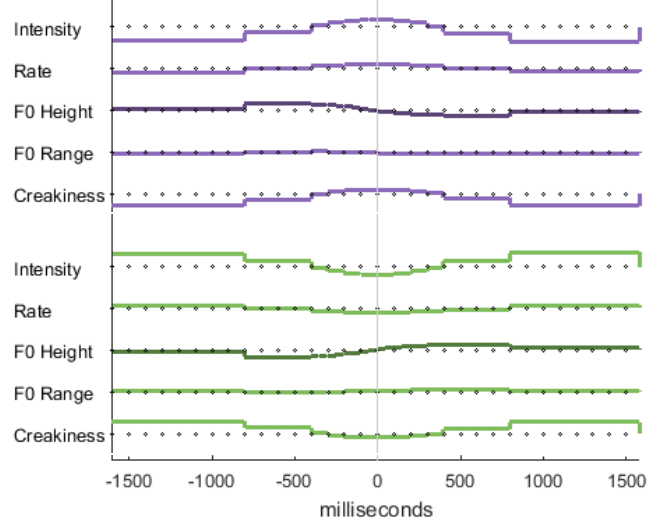
Figure 1: Loadings of Dimension 4. The top of the diagram (purple lines) shows the loadings for the left-track speaker, across the various features and windows, and the bottom half (green) the right-track speaker. Time is in milliseconds. The dotted lines are zeros, with points above them positively loaded and points below negatively loaded.
