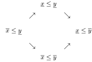
Fig. 5 Implications between truth values t_{\pm\pm}
