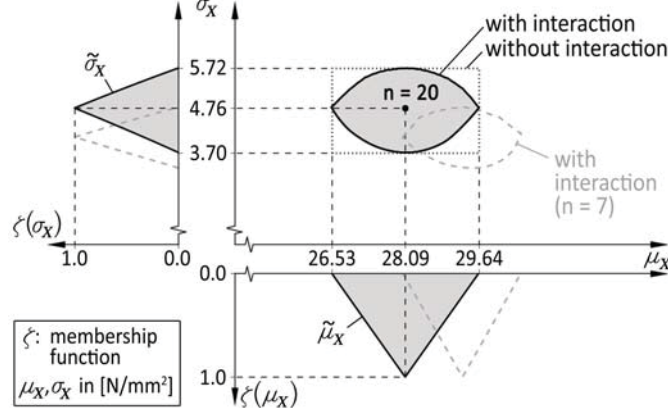
Figure 3: \mu_X – \sigma_X interaction after Bayesian update with imprecise data for the 2-D normal prior.
