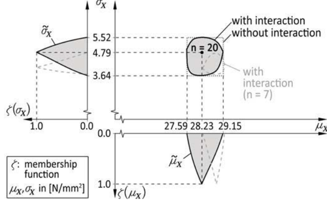
Figure 6: \mu_X - \sigma_X interaction after Bayesian update with imprecise data for the 2-D uniform prior.
